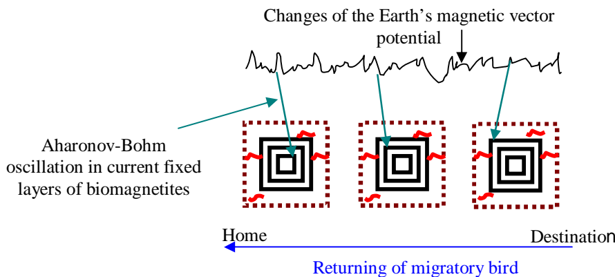
Fig. 3b. During return of bird, previously fixed vector potentials of Earth's magnetic fields can induce an Aharonov-Bohm type of oscillation in the fixed layer of biomagnetites. Therefore, the electric resistance of biomagnetites oscillates. Localized – previously fixed and spin-modulated – non-conductive electrons act as scattering sites for the mobile electrons. Namely, oscillations of dephasing non-conductive (fixed) electrons can have an influence on conductive mobile electrons in biomagnetites. Then, there is a coherent transport of mobile electrons' spins into surrounding semiconductor protein molecules. Finally, the oscillation of the electric resistance in biomagnetites as well as the transport of spins into proteins can induce conformational changes in organic proteins at the free rotations.
