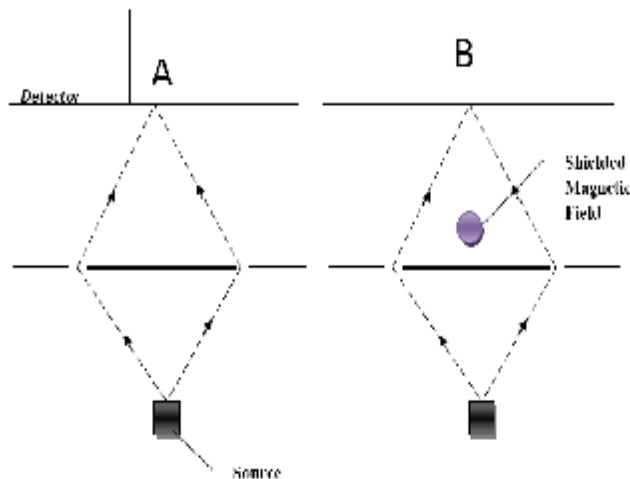
Fig. 2. Aharonov-Bohm effect: In the interference experiment for electron particles, in part A there is no any magnetic field around the set-up, but in part 2 there is a shielded magnetic field after the two-slit which has no any classical effect on the paths of electrons. The interference representations on detectors A and B are different. The magnetic field in part 2 has changed the wave phase of electrons.
