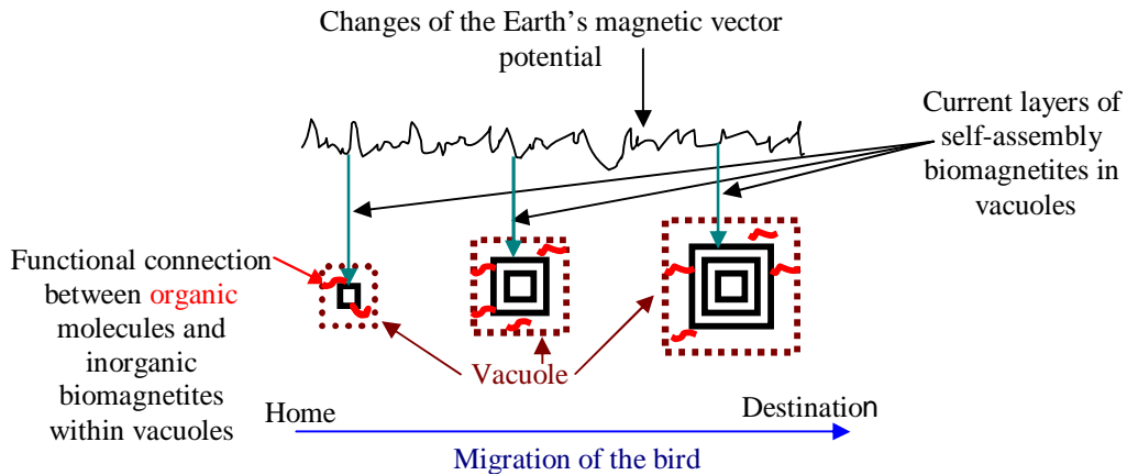
Fig. 3a. When the time of bird migration comes, migration intention can induce a genetic program in brain cells of migratory birds, which initiates and operates the development of biomagnetites in vacuoles. During migration, layers of biomagnetites and phases of non-conductive electrons in the layers are shaped by current magnetic vector potential field of Earth (Fig.1a). These polarized states of non-conductive electrons – which ones are fixed in current layers in biomagnetites – can play the main role in magnetic information storage.
